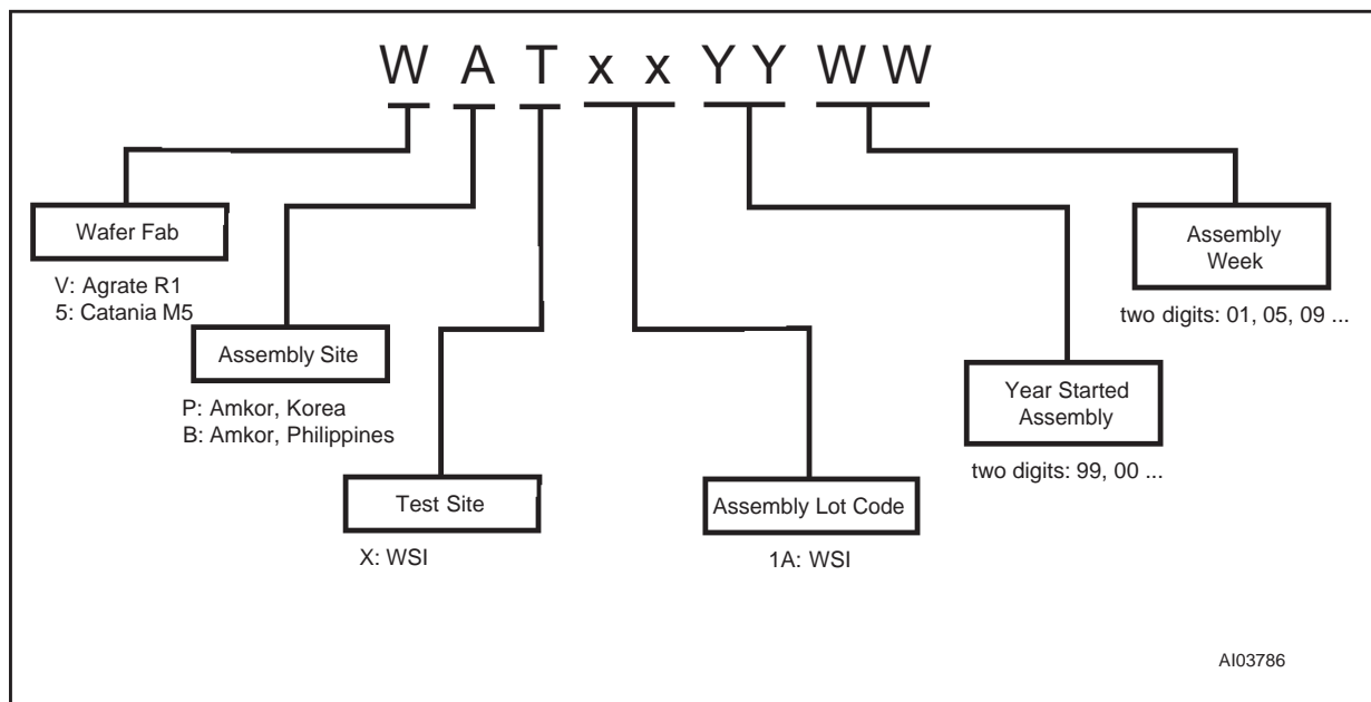
Figure 2. Trace Code
