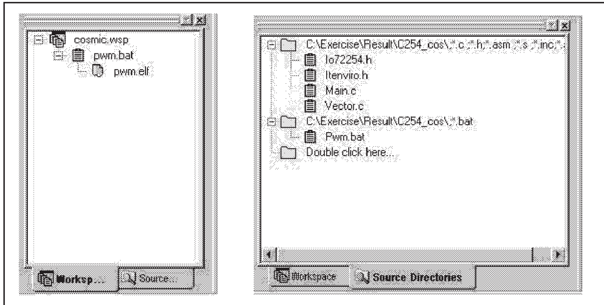
Figure 3. Workspace Window
