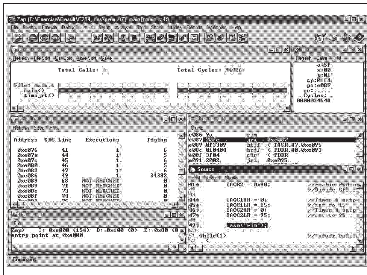
Figure 1. ZAP Simulator
