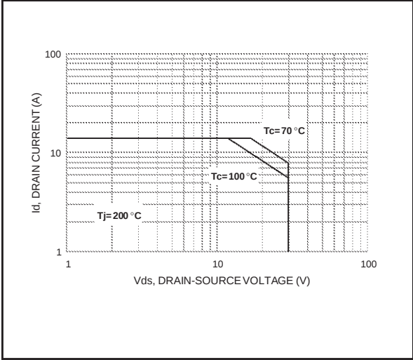
DC Safe Operating Area
