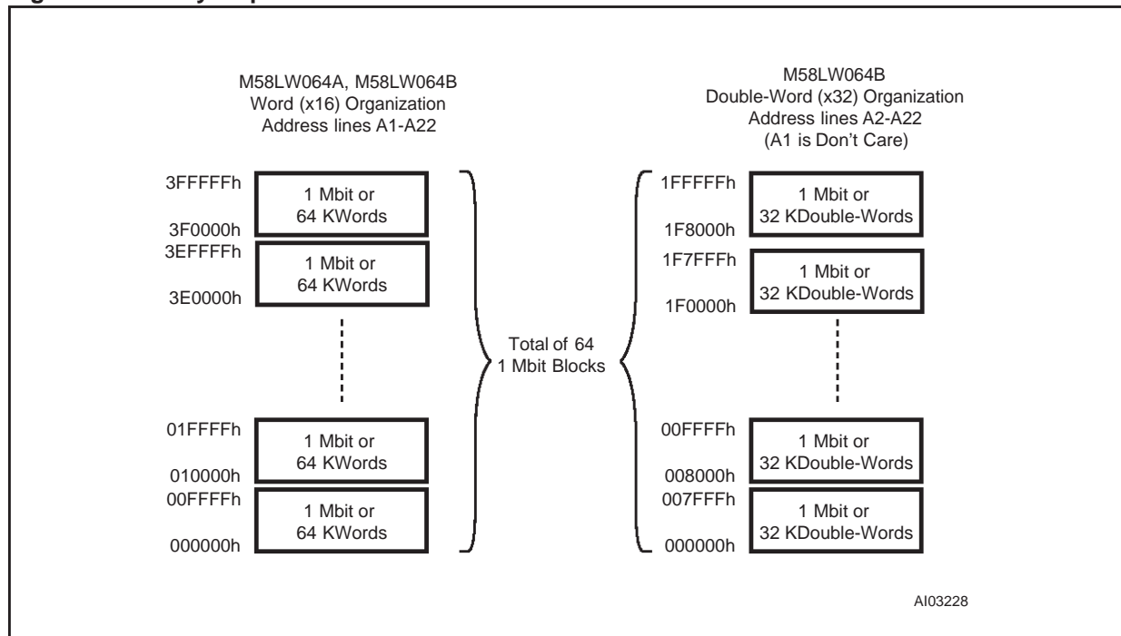
Figure 6. Memory Map
