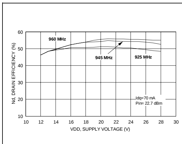
Drain Efficiency vs. Supply Voltage
