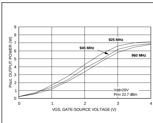
Output Power vs. Gate-Source Voltage
