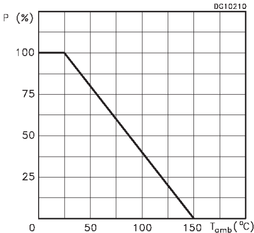
Derating Curve
