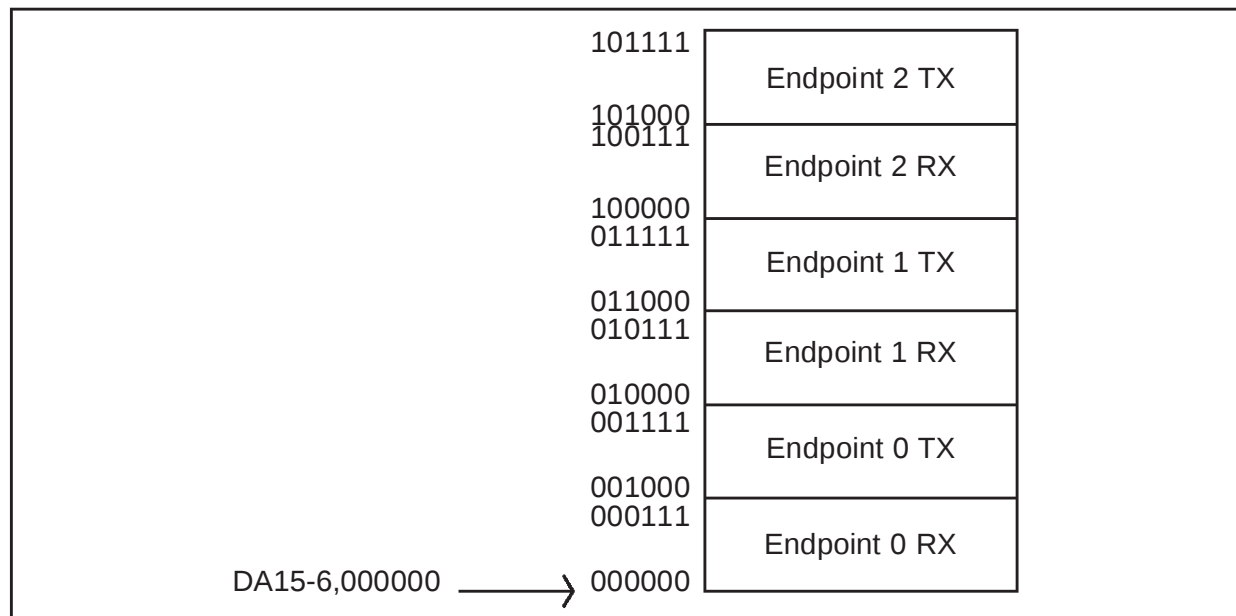
Figure 26. DMA Buffers
