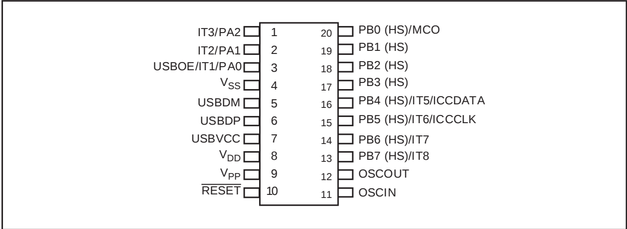
Figure 2. 20-pin SO20 Package Pinout
