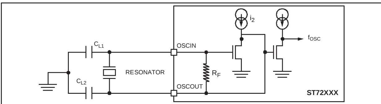
Figure 33. Typical Application with a Crystal Resonator
