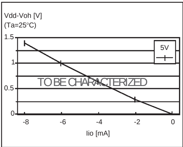
Figure 48. Typical V_{DD}-V_{OH} at V_{DD}=5V
