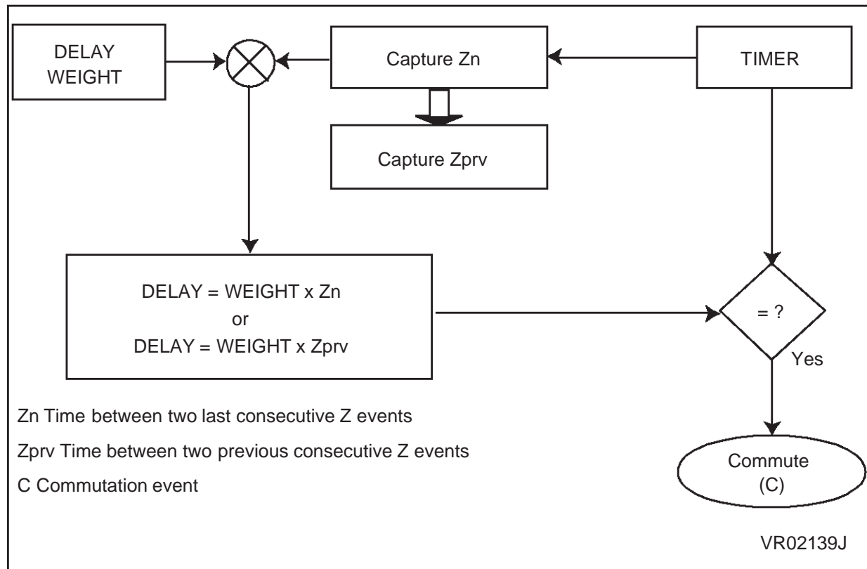
Figure 11. Delay manager
