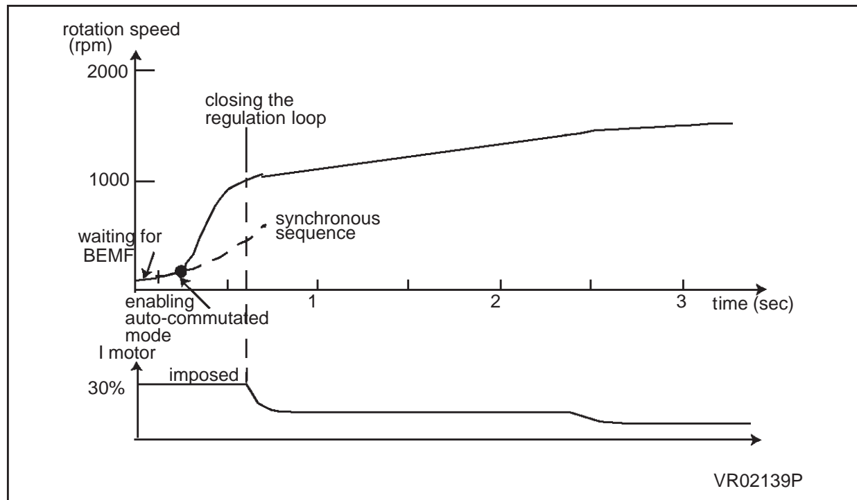
Figure 17. Starting sequence
