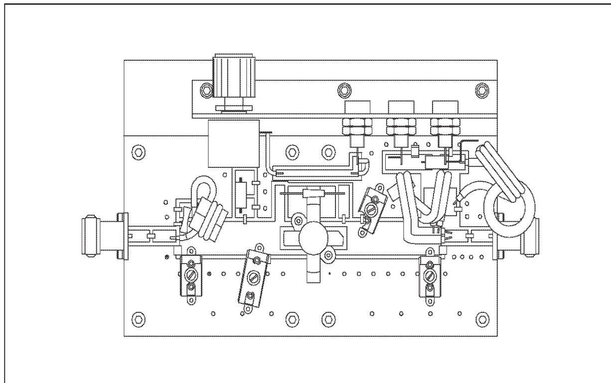
175 MHz Test Circuit
