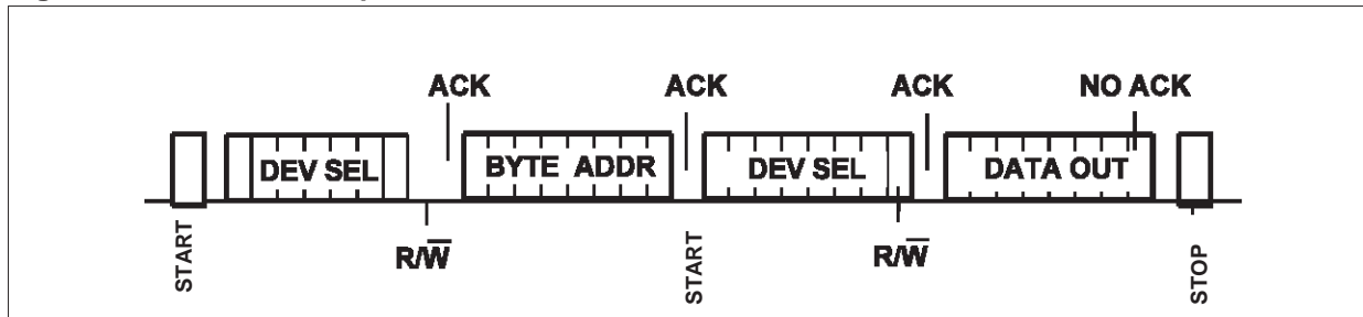
Figure 4 - Read Mode Sequence
