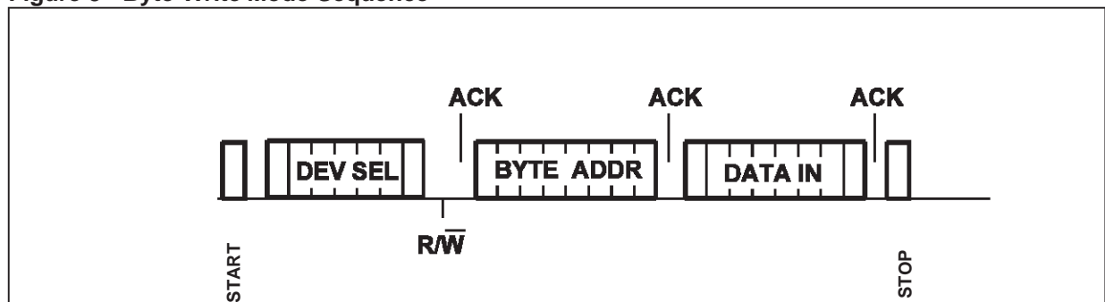
Figure 3 - Byte Write Mode Sequence
