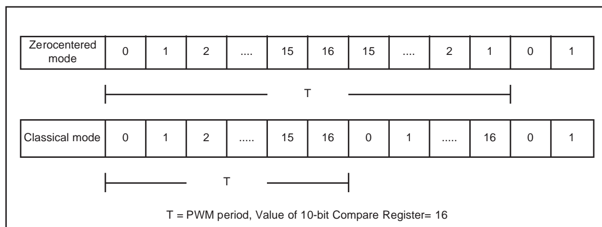
Figure 63. Counting sequence in Zero-centered and Classical mode
