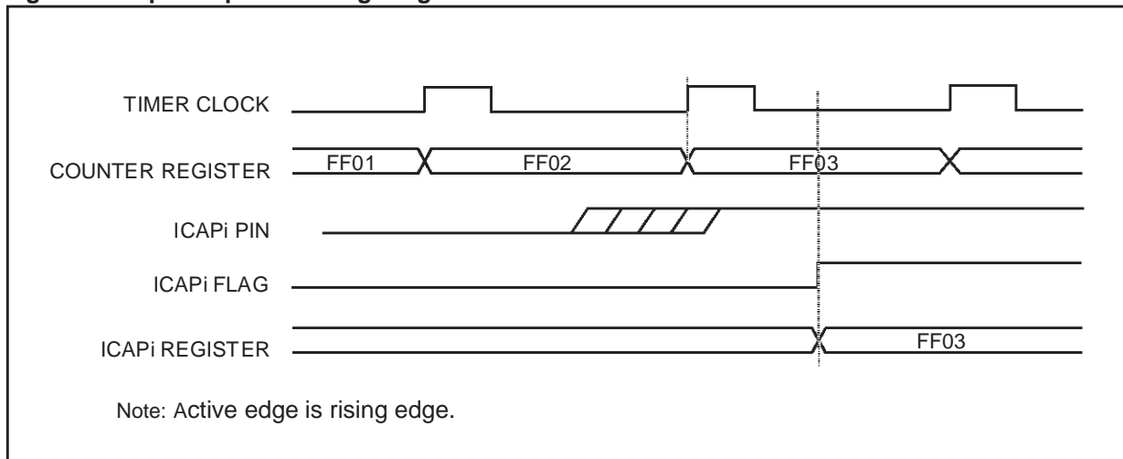
Figure 57. Input Capture Timing Diagram
