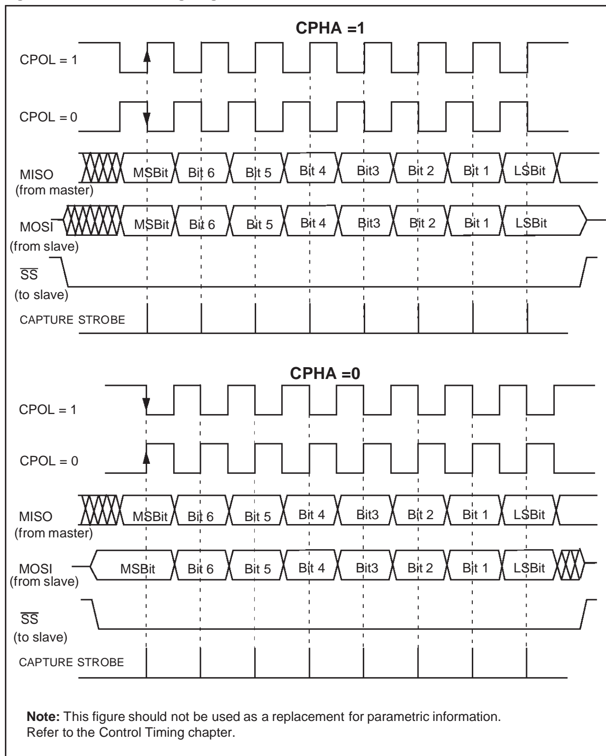
Figure 74. Data Clock Timing Diagram
