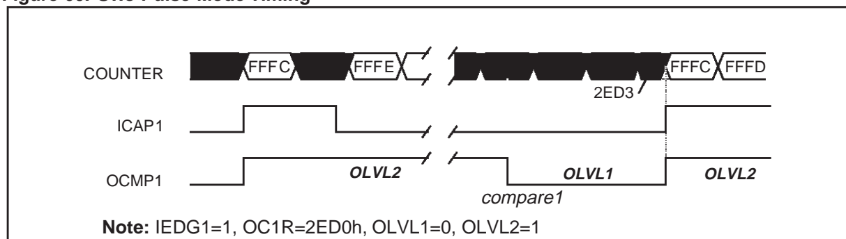
Figure 60. One Pulse Mode Timing
