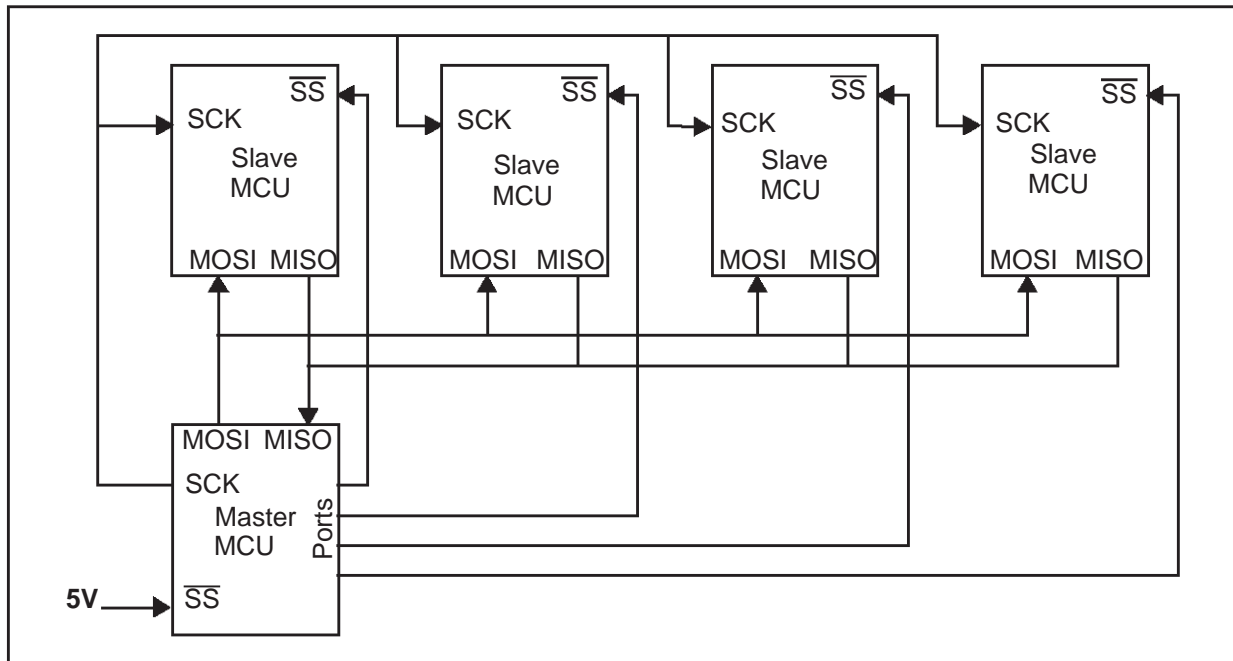
Figure 76. Single Master Configuration
