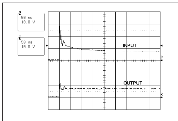
Fig. A5: Remaining voltage at the input and output of the device during a \pm 16\text{kV} ESD surge (IEC61000-4-2).
