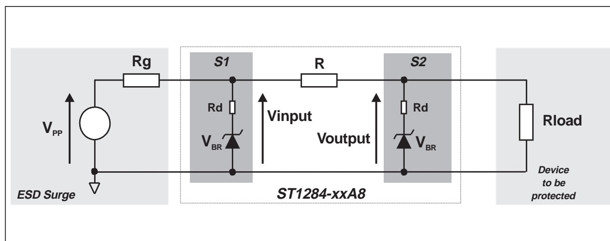
Fig. A3: ST1284 ESD clamping behavior
