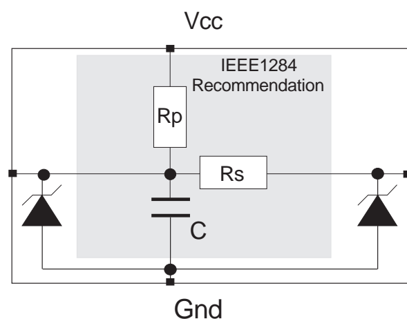
Fig. 1: Cell 1 for line termination, EMI filtering and ESD protection for the Datalines and Strobe signals. This cell is present 9 times inside the ST1284-xxA8
