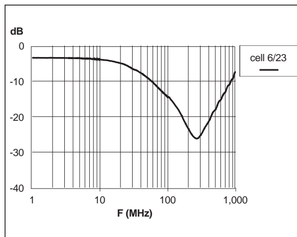
Fig. A2: Frequency response curve for data and strobe signals.
