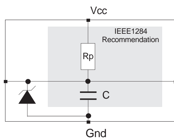
Fig. 2: Cell 2 for EMI filtering and ESD protection of the Control and Status signals. This cell is present 8 times inside the ST1284-xxA8
