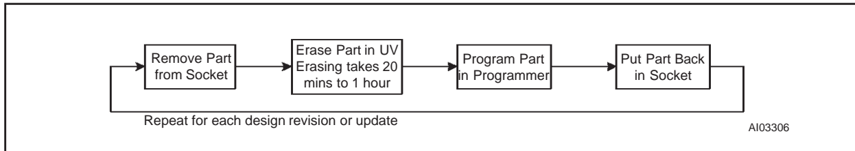
Figure 2. Design Cycle for a Windowed Eprom-Based Part
