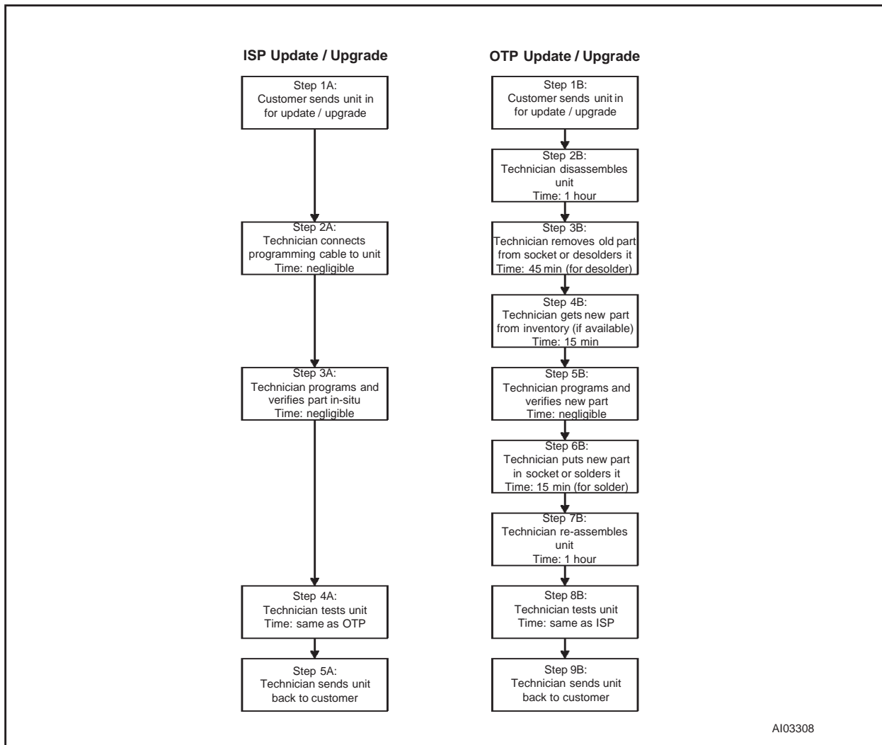
Figure 4. ISP update/upgrade versus OTP update/upgrade
