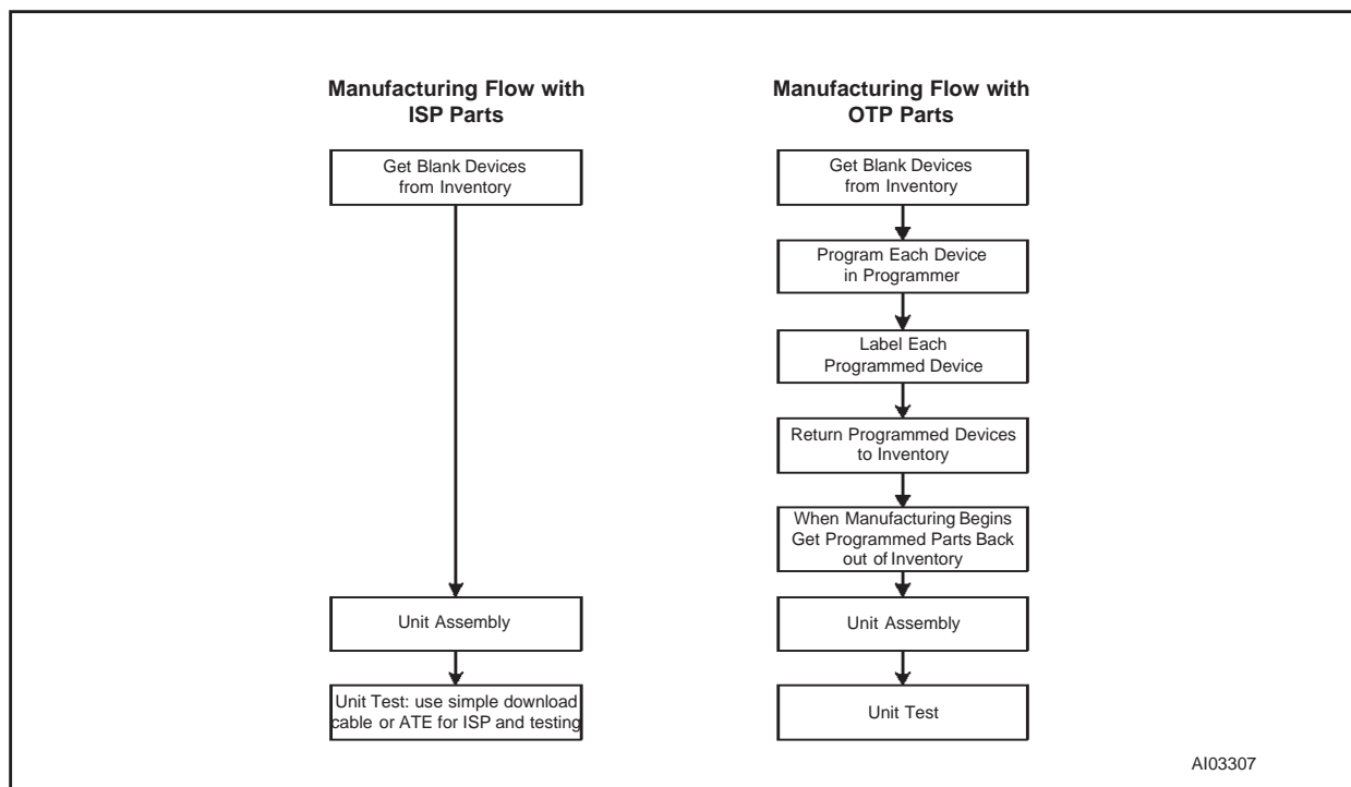
Figure 3. Manufacturing Flow with ISP versus OTP parts
