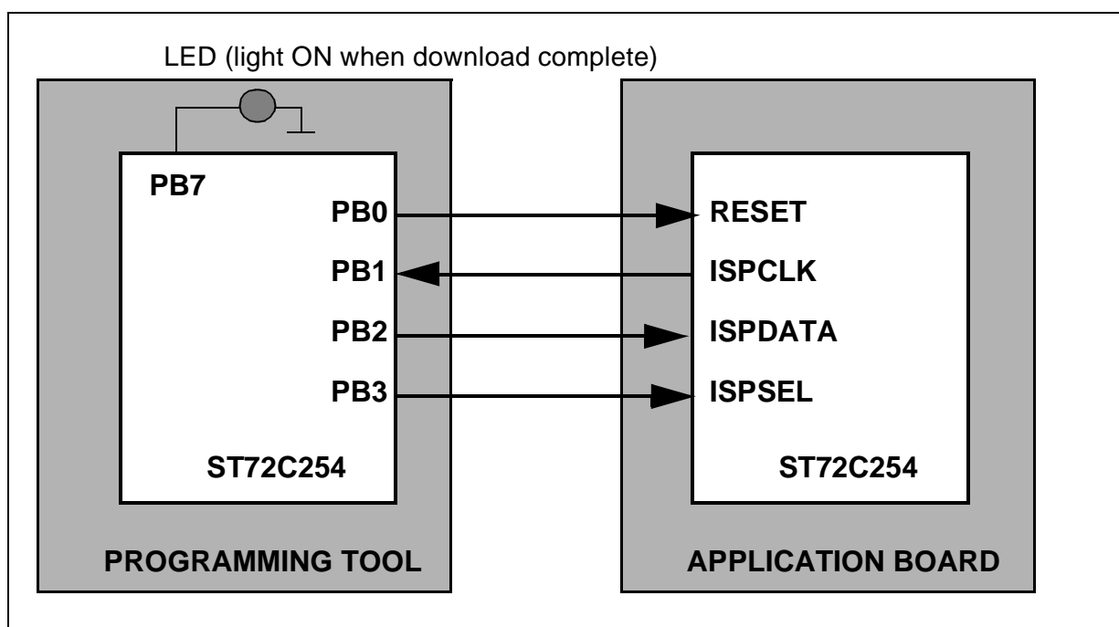
Figure 11. Application Circuit
