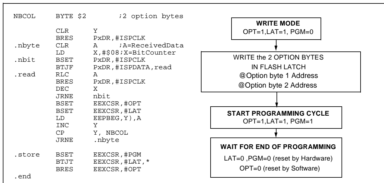
Figure 9. Option Bytes Programming Code & Flowchart
