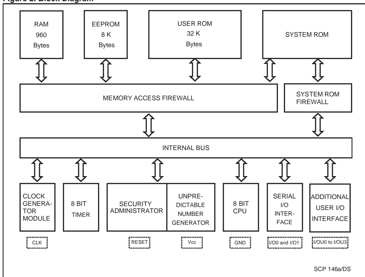
Figure 2. Block Diagram
