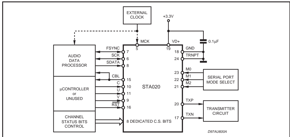
Figure 2. STA020 Typical Connection Diagram.
