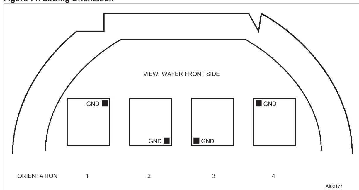
Figure 11. Sawing Orientation
