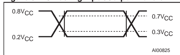
Figure 8. AC Testing Input/Output Waveform
