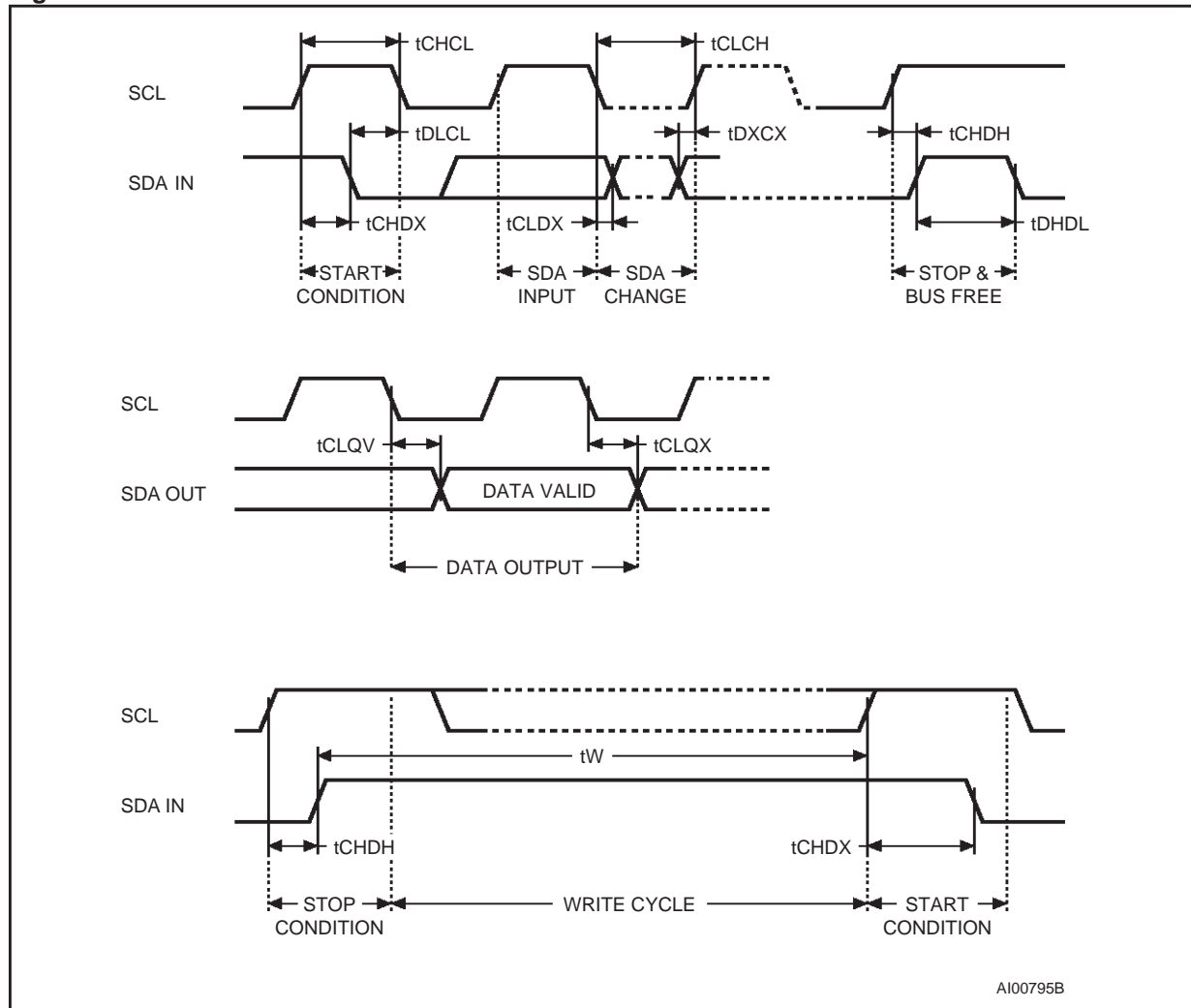
Figure 9. AC Waveforms
