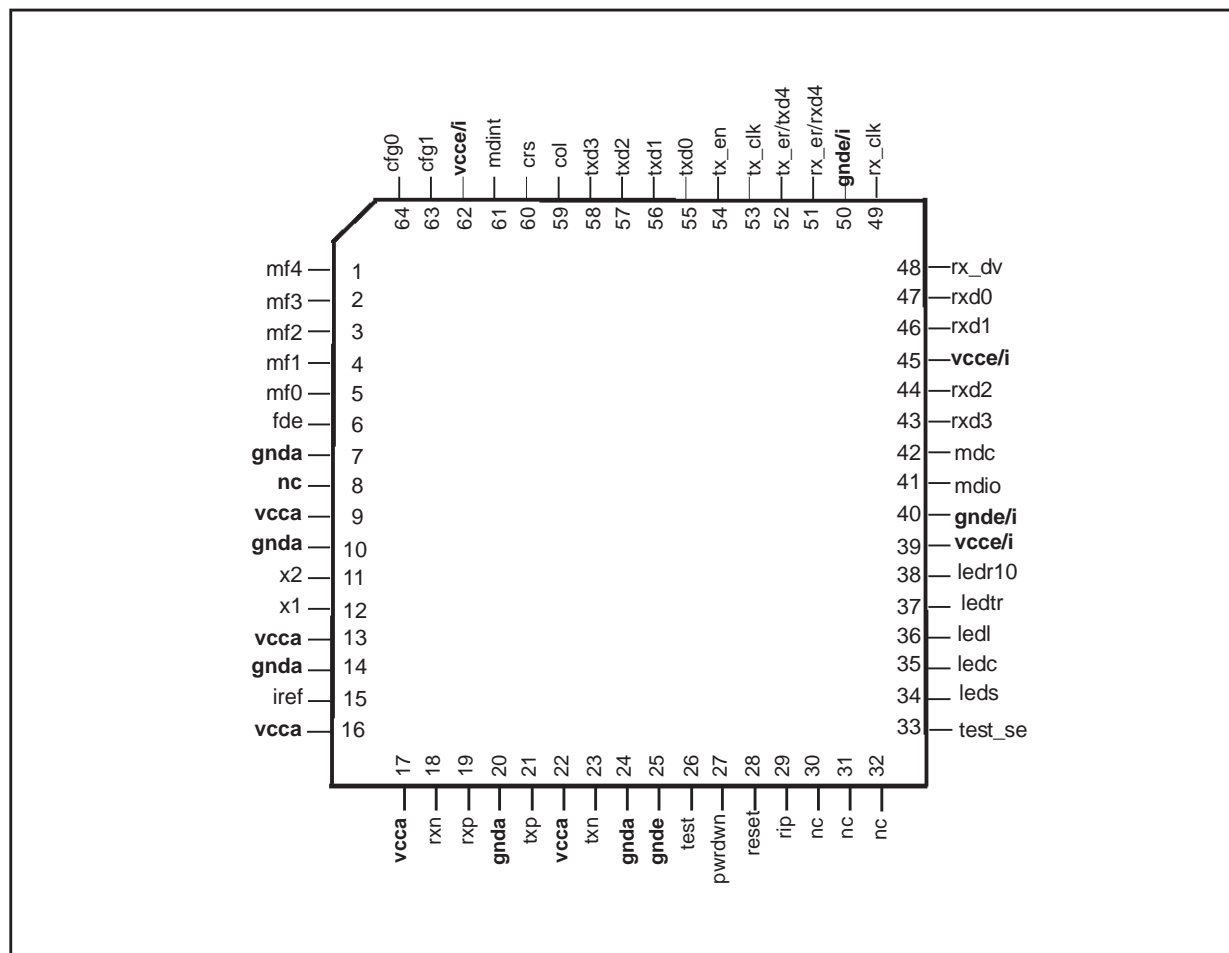
Figure 3. Pin Connection
