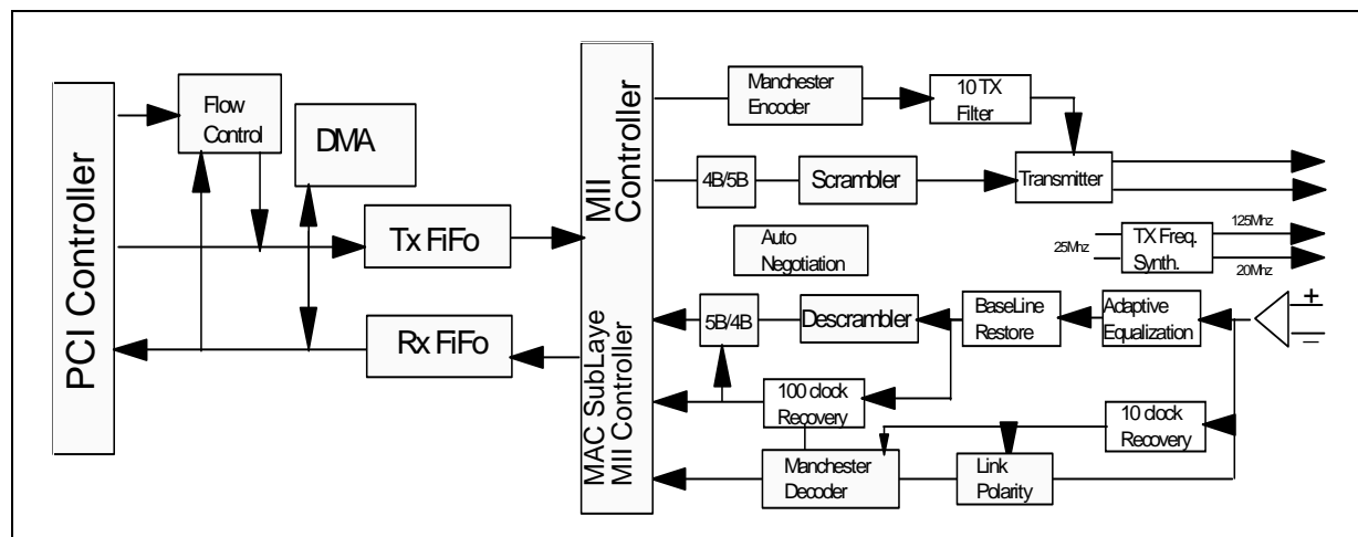
Figure 1. STE10/100A Block Diagram
