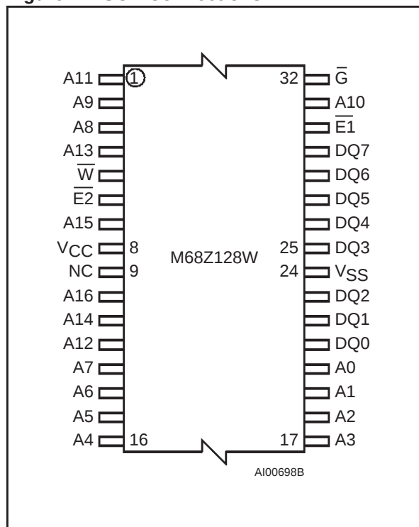
Figure 2. TSOP Connections
