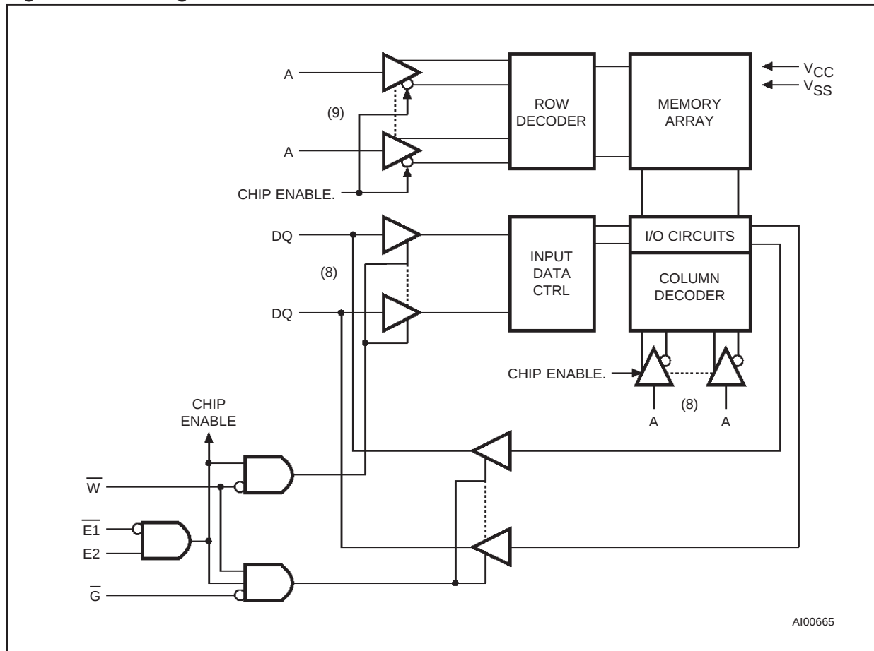
Figure 4. Block Diagram
