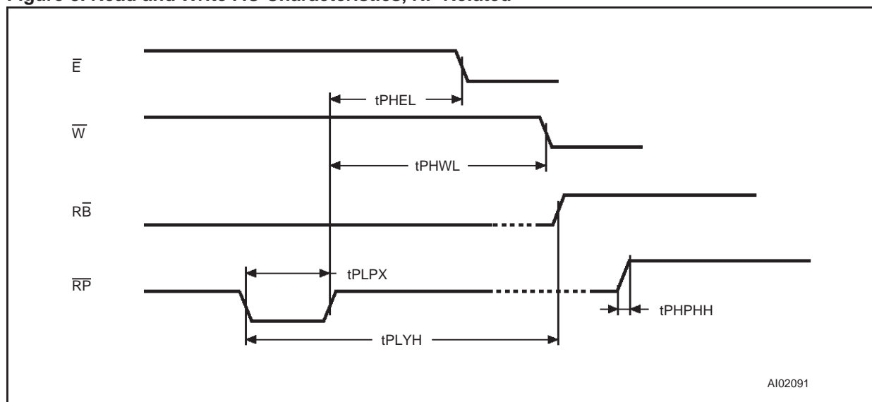
Figure 8. Read and Write AC Characteristics, \overline{RP} Related
