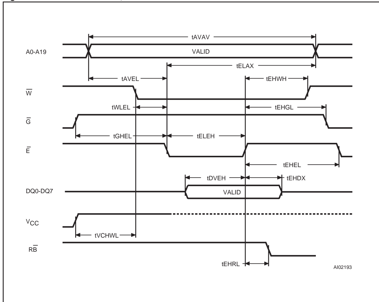
Figure 7. Write AC Waveforms, \overline{E} Controlled
