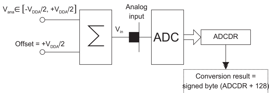
Measuring relative voltages using an analog offset
