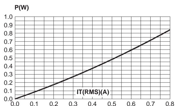
Fig. 5: Maximum power dissipation versus RMS on-state current.
