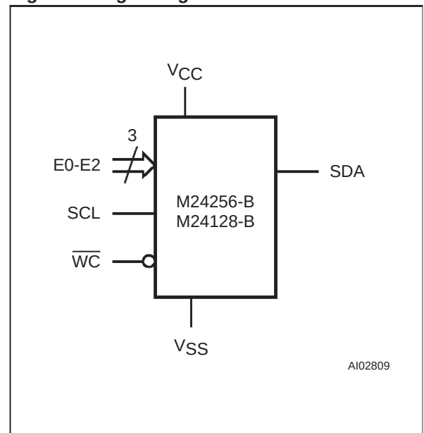
Figure 1. Logic Diagram
