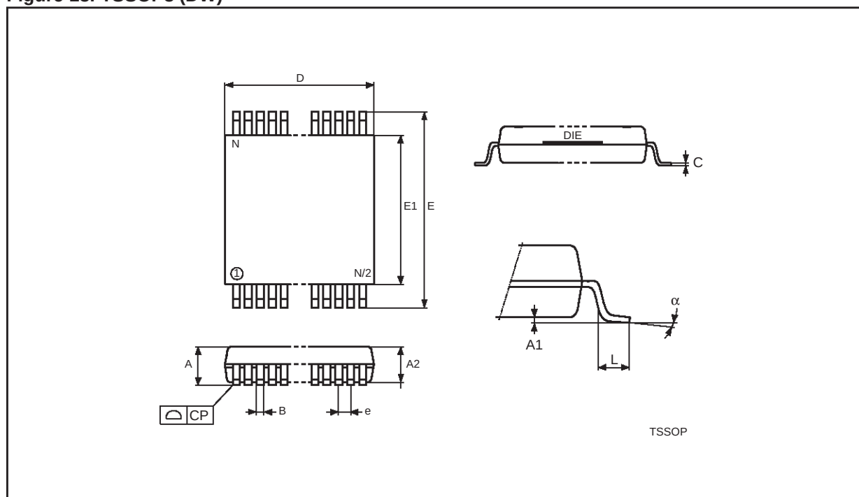
Figure 13. TSSOP8 (DW)
