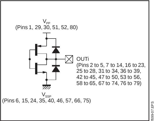
Figure 5 : Power Output
