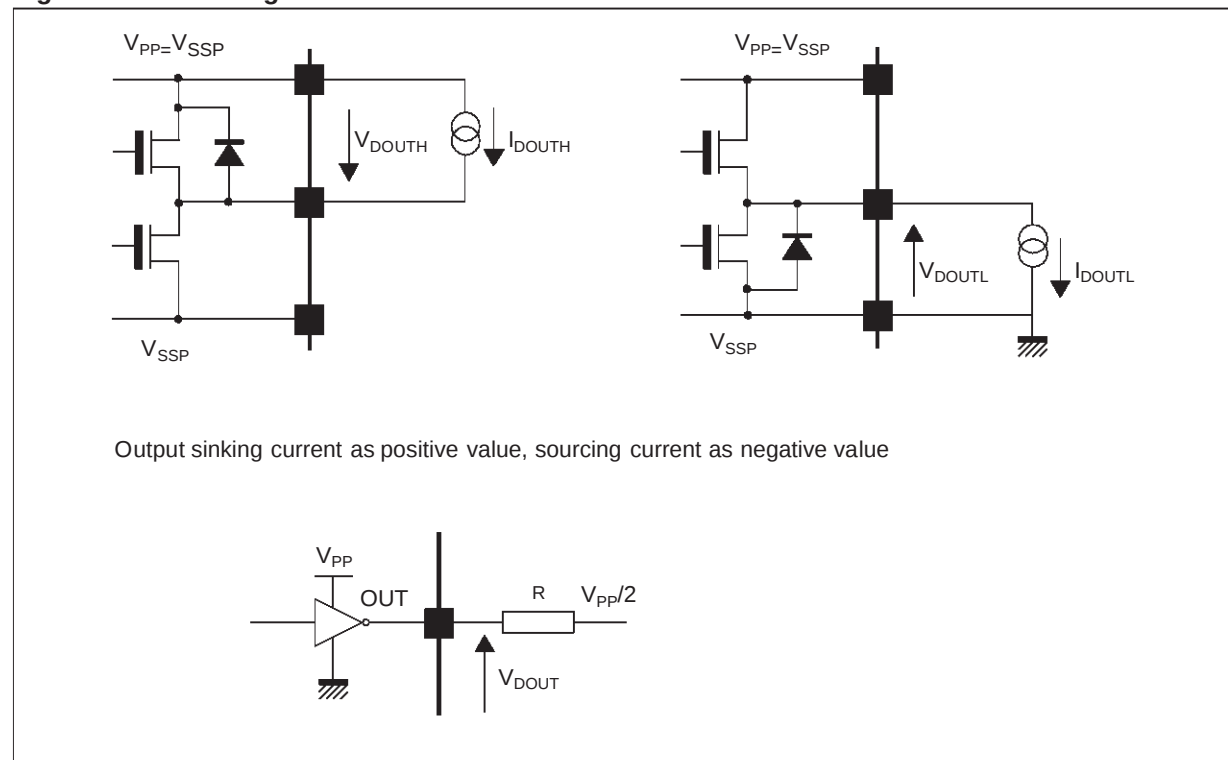
Figure 2: Test Configuration
