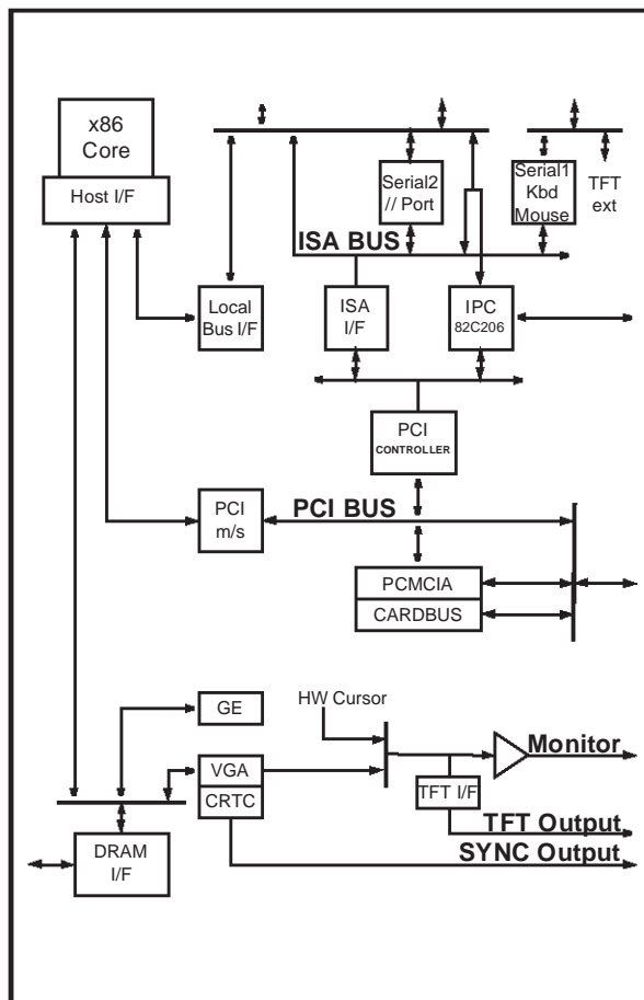
Figure 1. Logic Diagram
