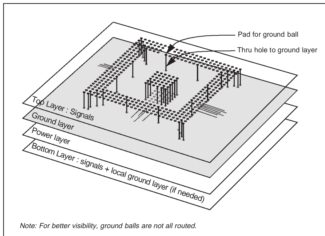
Figure 6-1. Ground routing
