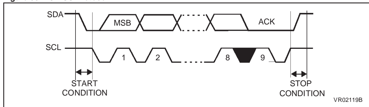
Figure 38. I C BUS Protocol
