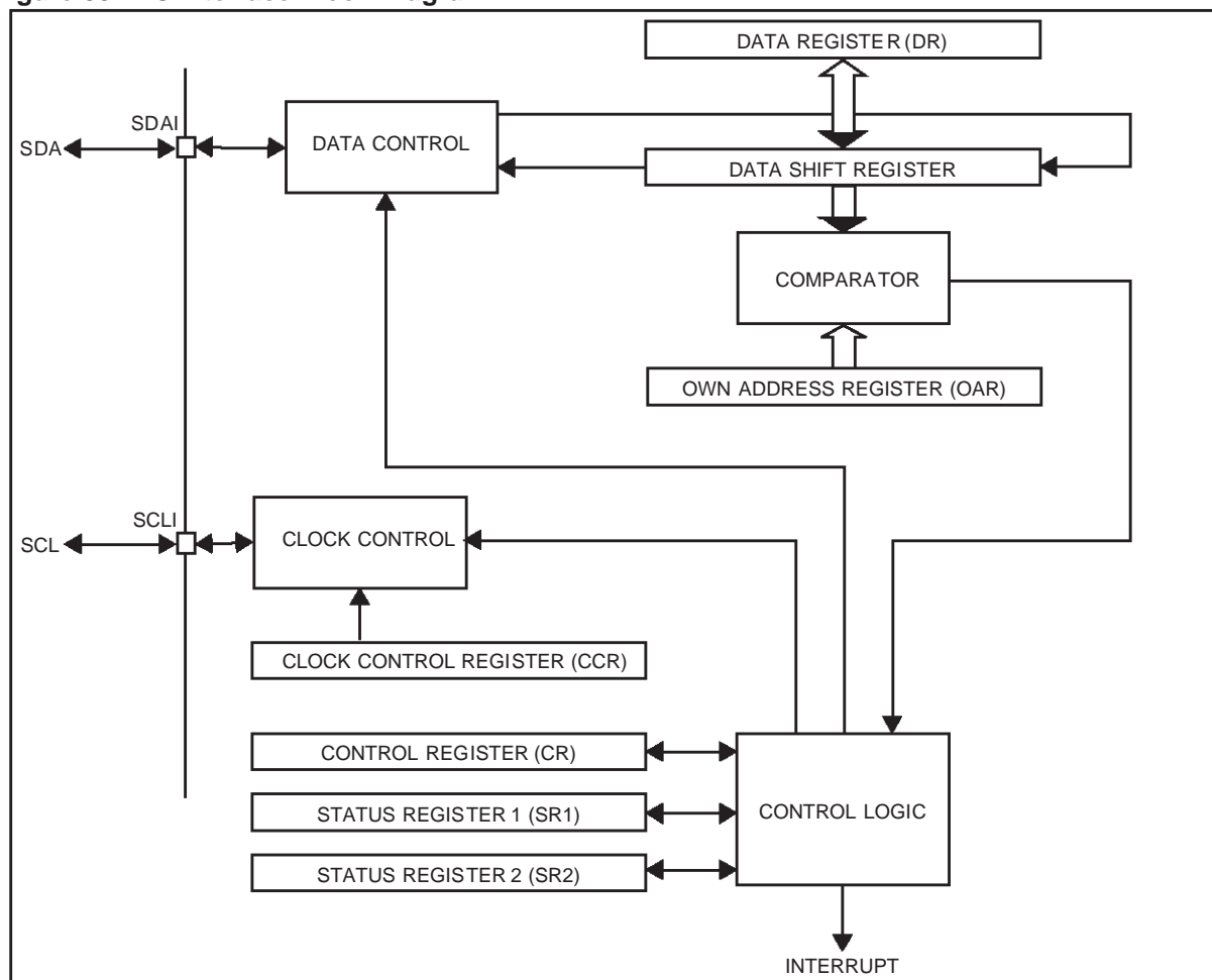
Figure 39. I C Interface Block Diagram
