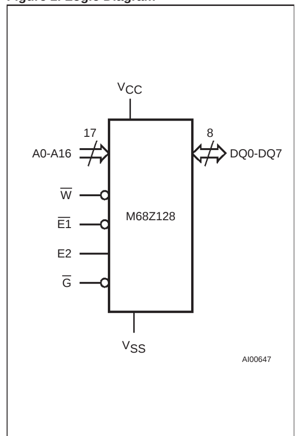
Figure 1. Logic Diagram
