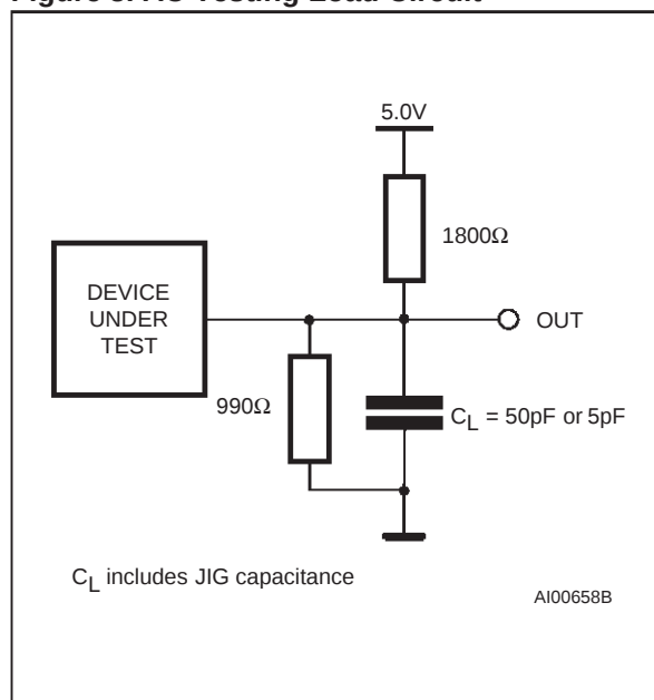
Figure 3. AC Testing Load Circuit
