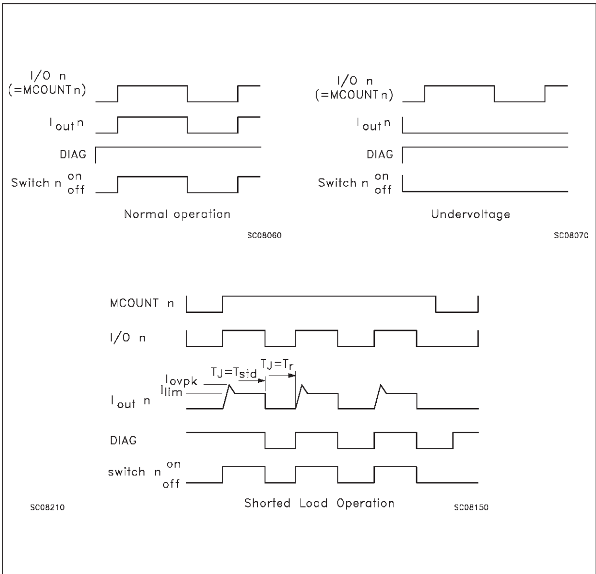
FIGURE 3: Switching Waveforms
