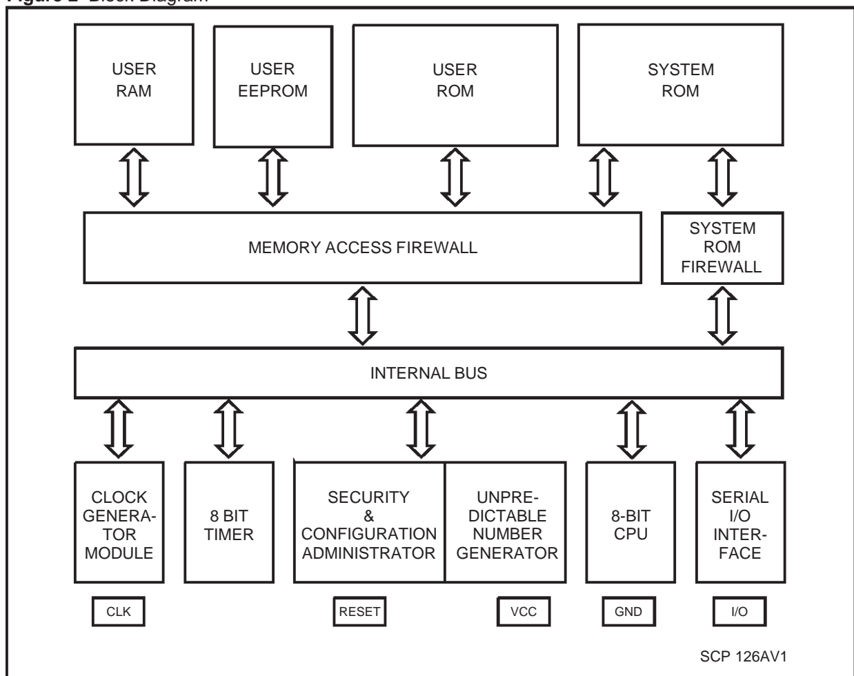
Figure 2 Block Diagram
