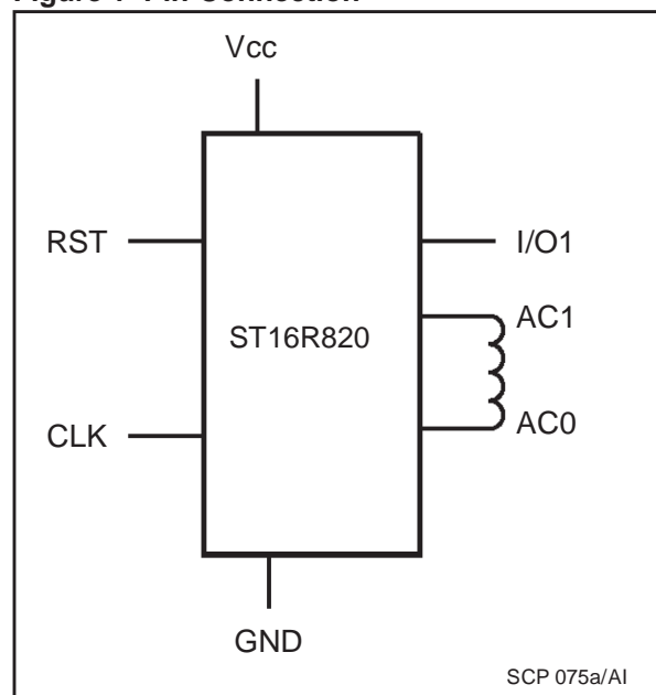
Figure 1 Pin Connection
