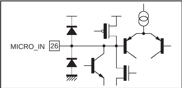
Figure 15 : MICRO_IN
