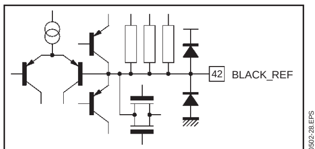
Figure 26 : BLACK_REF
