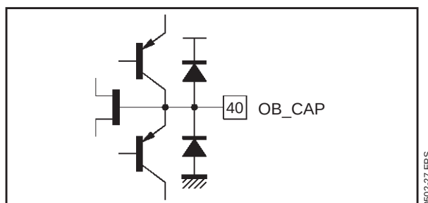
Figure 25 : OB_CAP
