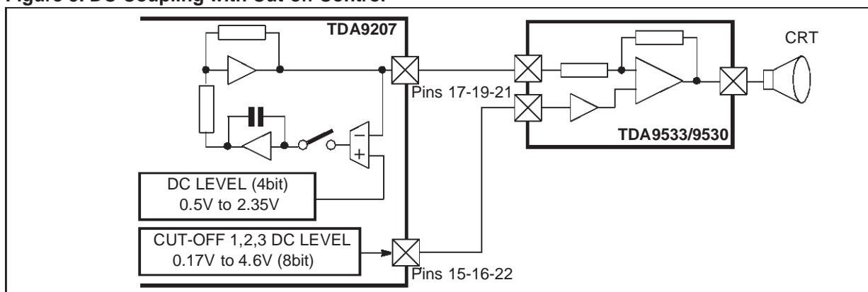
Figure 6. DC Coupling
