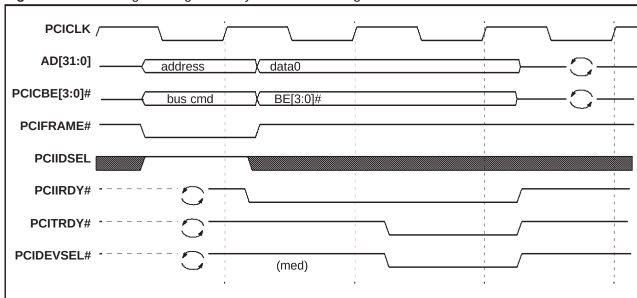
Figure 24. PCI Target configuration cycle - Slave Configuration Write
