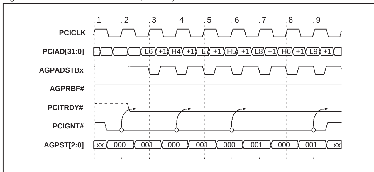
Figure 9. 2X Back to back read data, no delay
