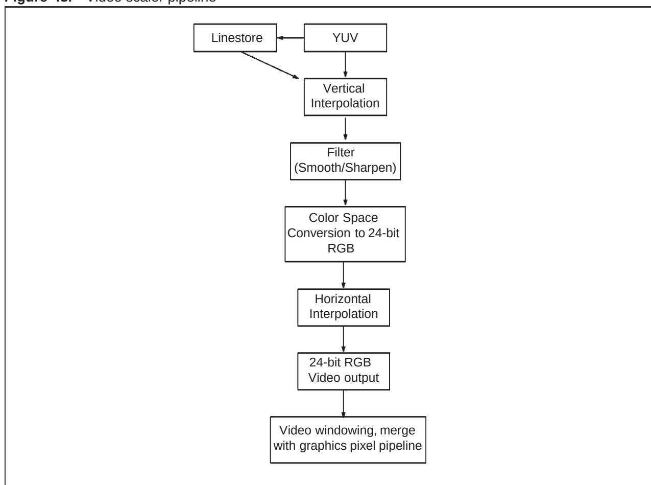
Figure 43. Video scaler pipeline
