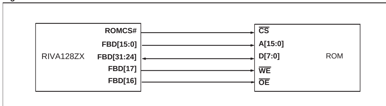
Figure 63. ROM interface
