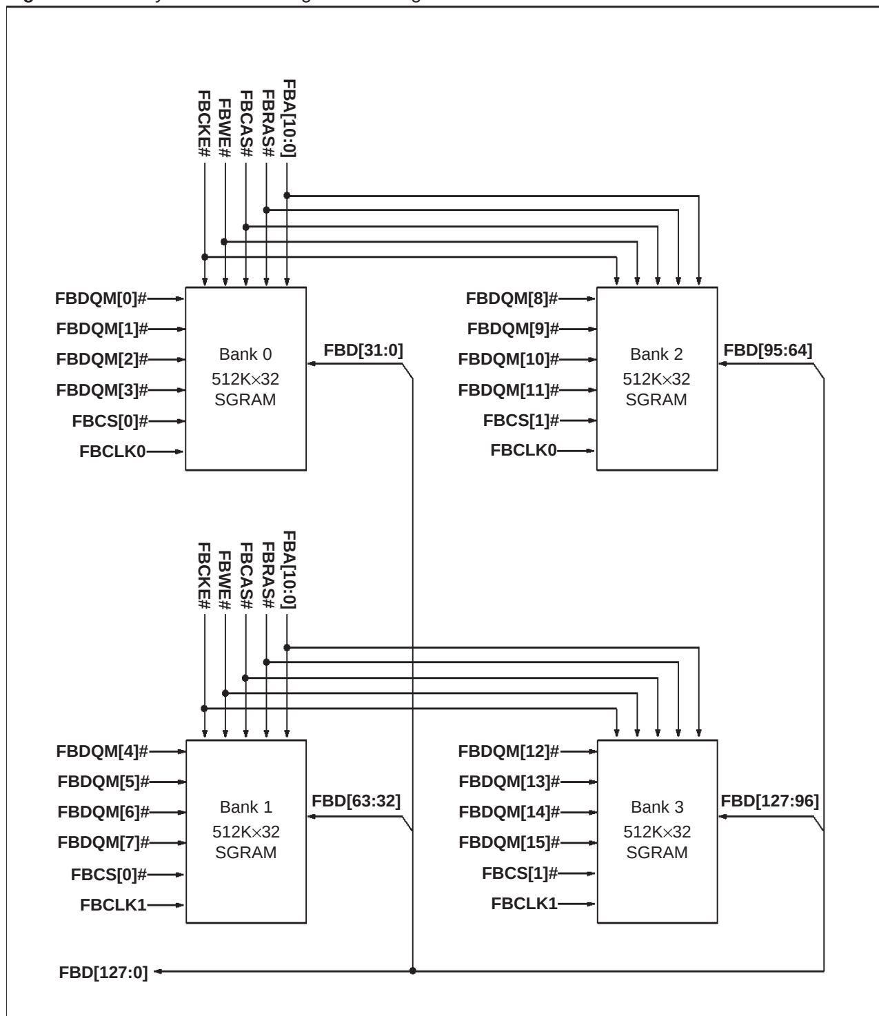
Figure 31. 8MByte SGRAM configuration using 16Mbit devices
