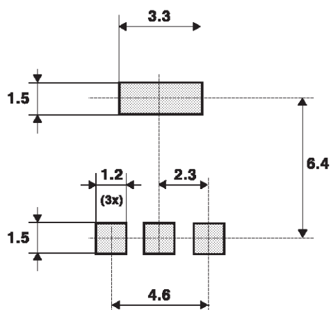
Recommended soldering pattern SOT223
