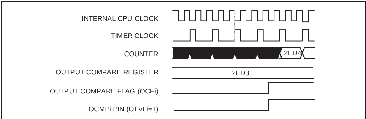
Figure 28. Output Compare Timing Diagram, Internal Clock Divided by 2
