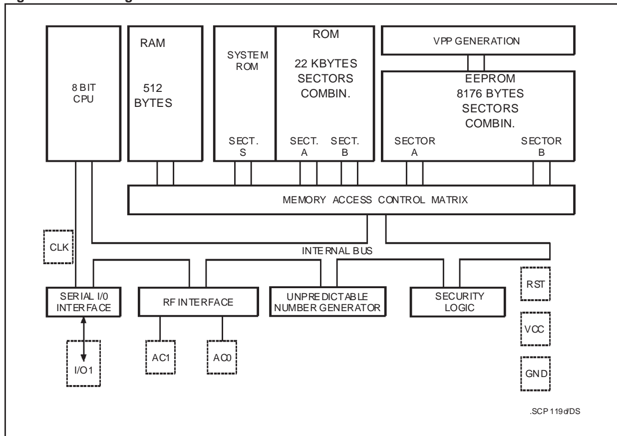
Figure 2 Block Diagram
