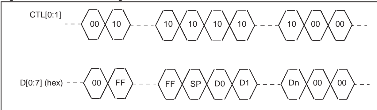
Figure 2.13 Receive timing
