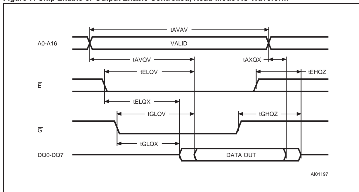
Figure 7. Chip Enable or Output Enable Controlled, Read Mode AC Waveform
