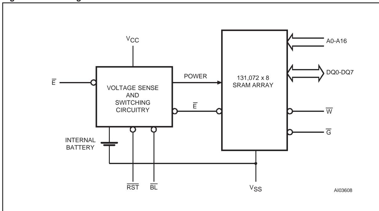
Figure 3. Block Diagram
