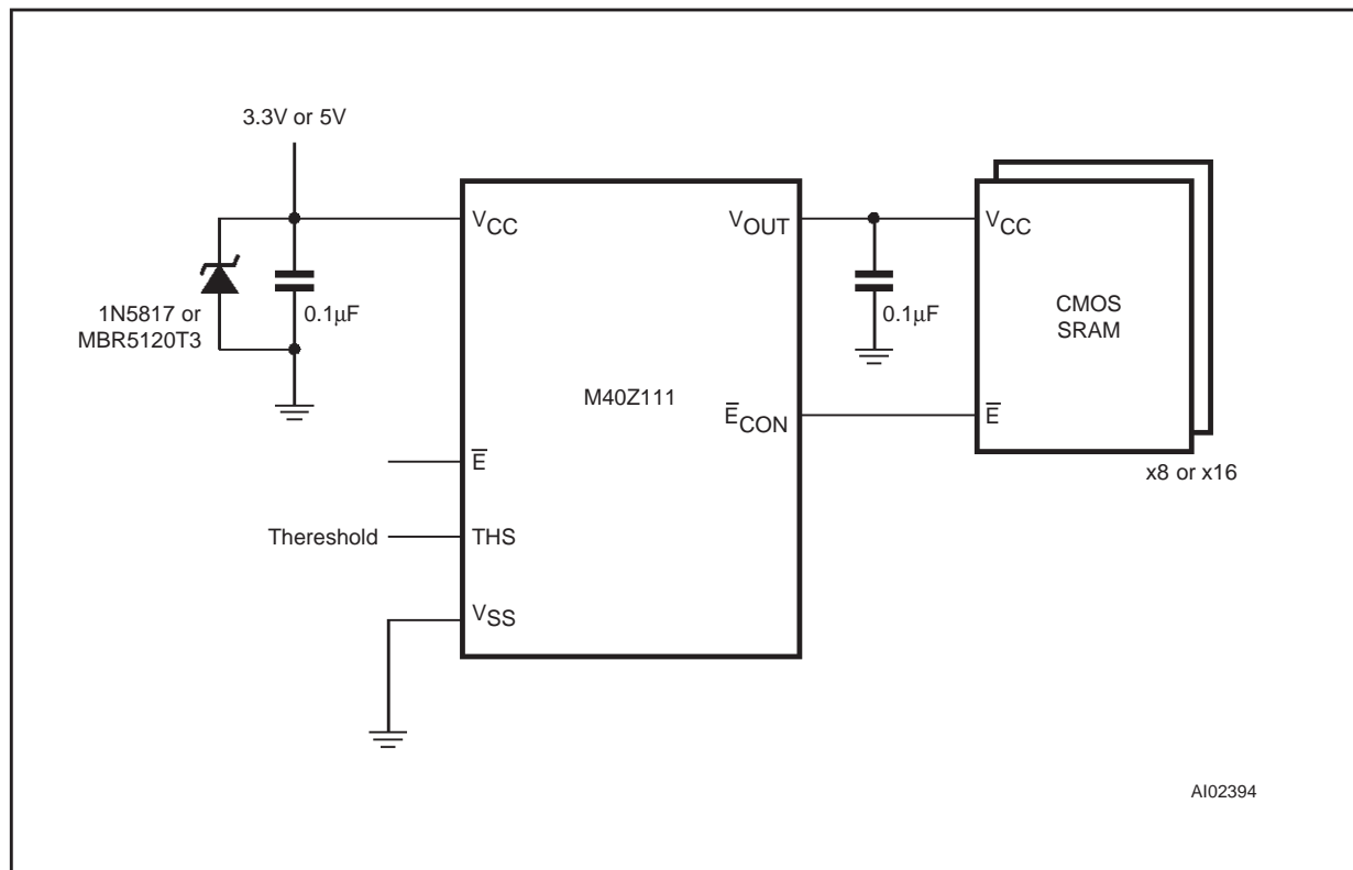
Figure 3. Hardware Hookup
