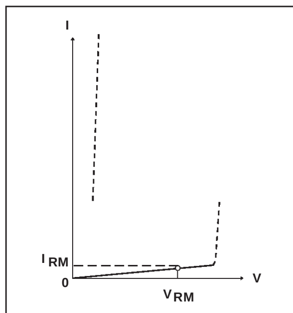
Figure 2 : Stand by Characteristics.
