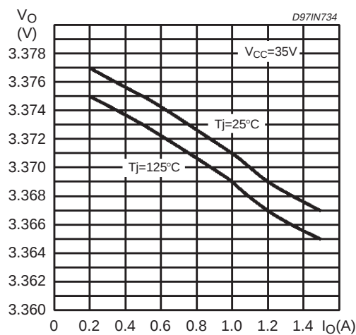
Figure 7. Load regulation
