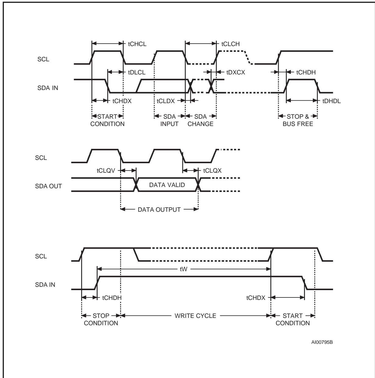
Figure 5. AC Waveforms
