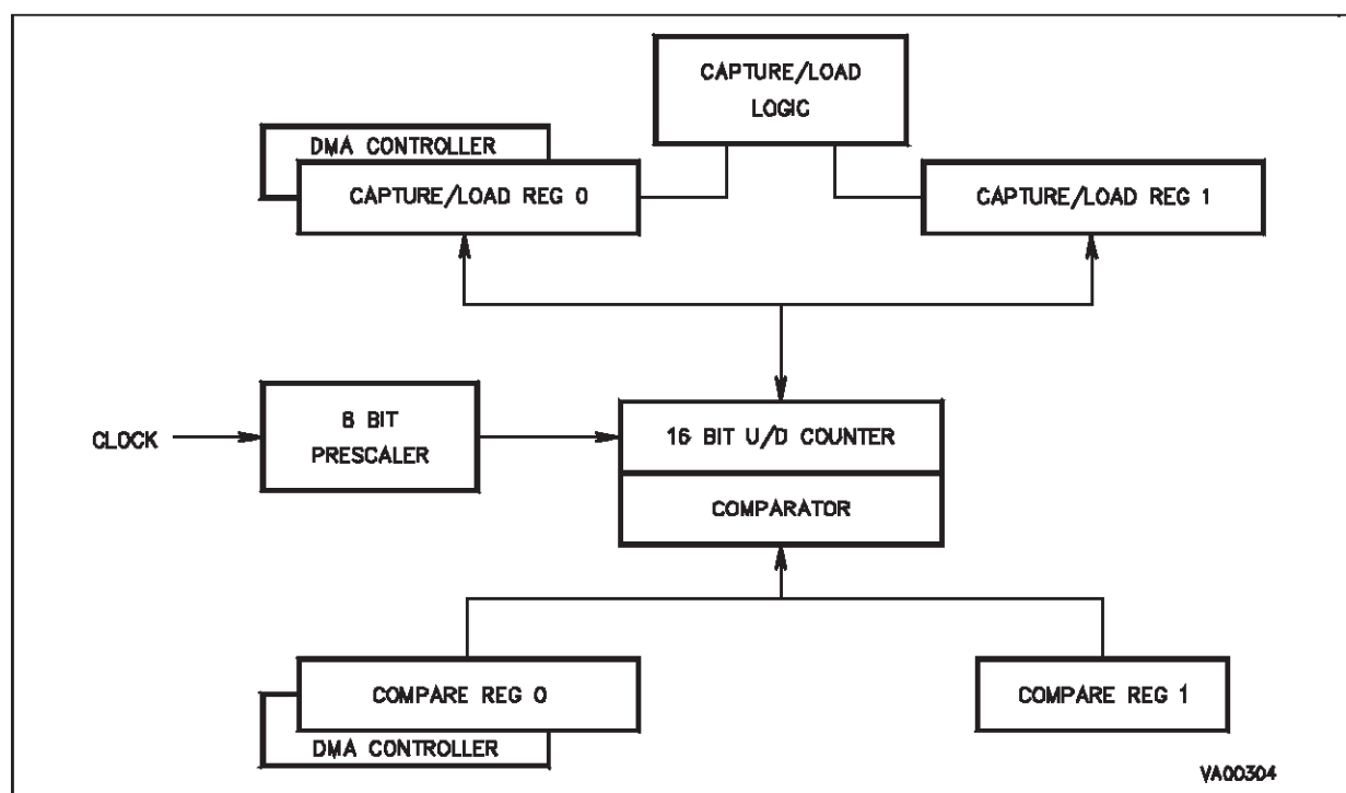
Figure 64. MFT Simplified Block Diagram
