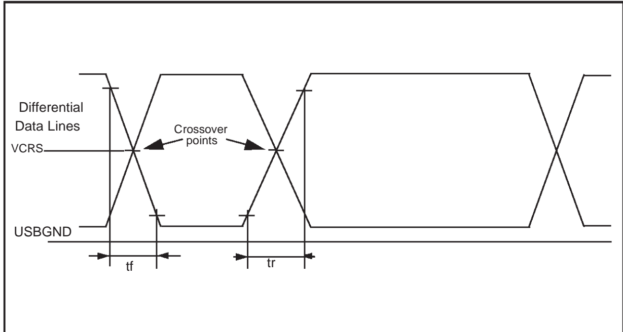
Figure 88. USB Interface: Data signal rise and fall time
