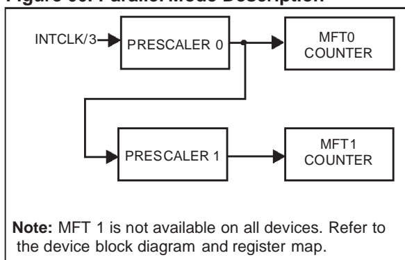
Figure 66. Parallel Mode Description
