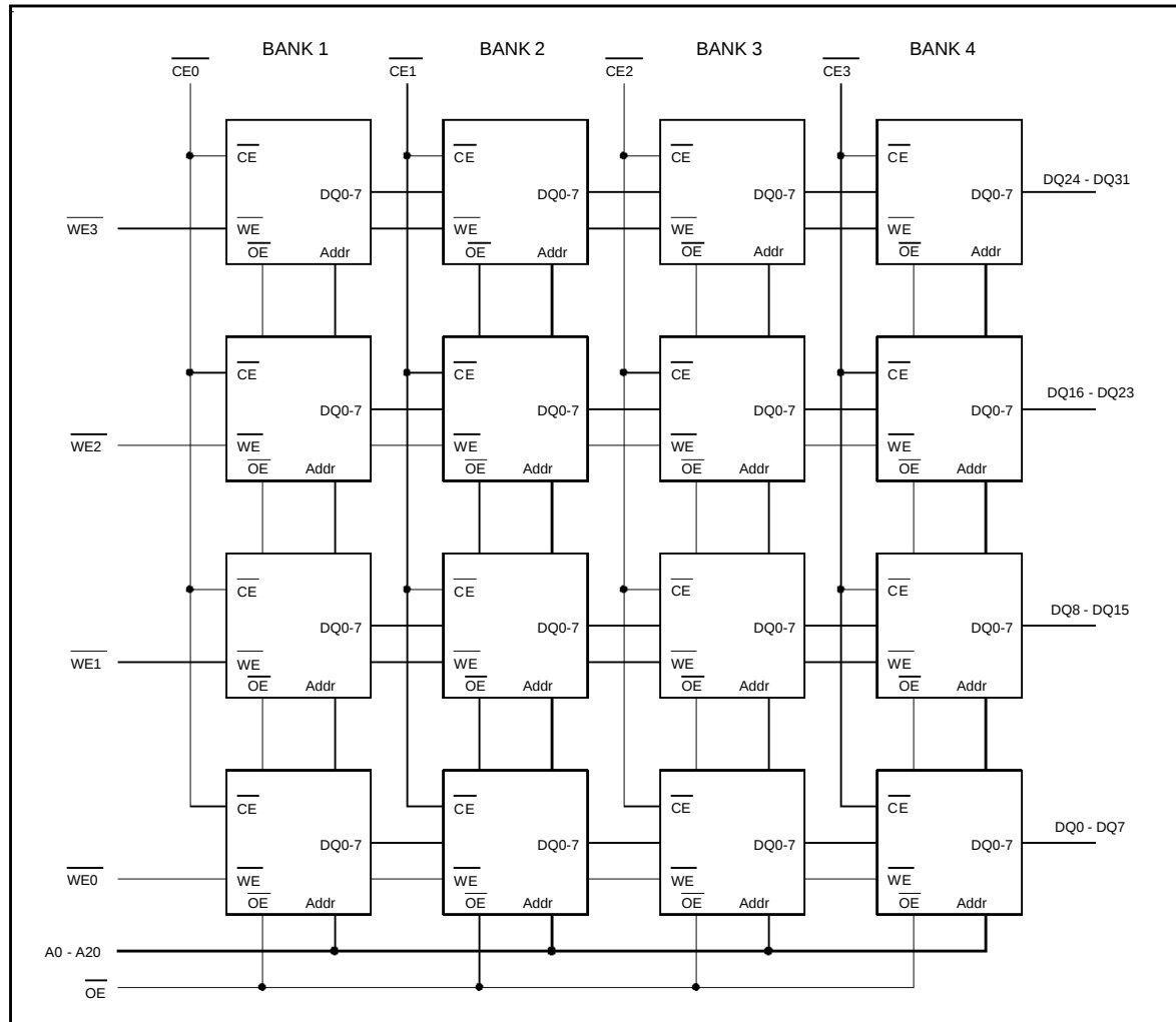
Fig. 1. Block diagram
