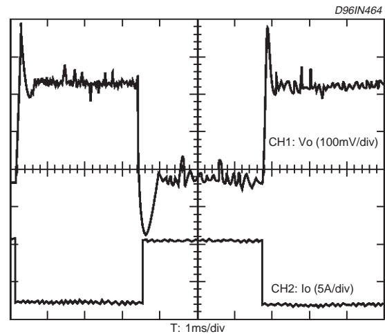
Figure 8a: Output voltage response versus load Fig 8b. Enlarged section of load
