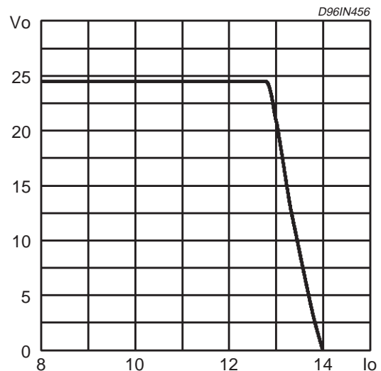
Figure 2: Output limiting current characteristic using two current transformers
