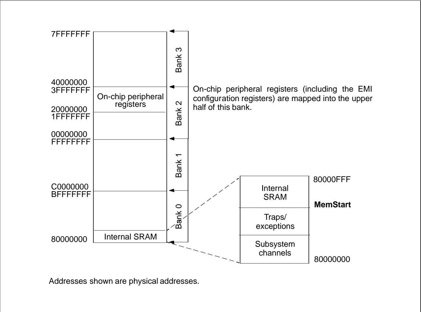
Figure 9.1 Memory allocation
