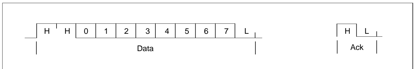
Figure 12.1 OS-Link data and acknowledge formats
